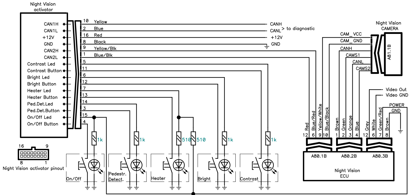
Pict 2. BMW FXX NiVi System Connection Diagram
