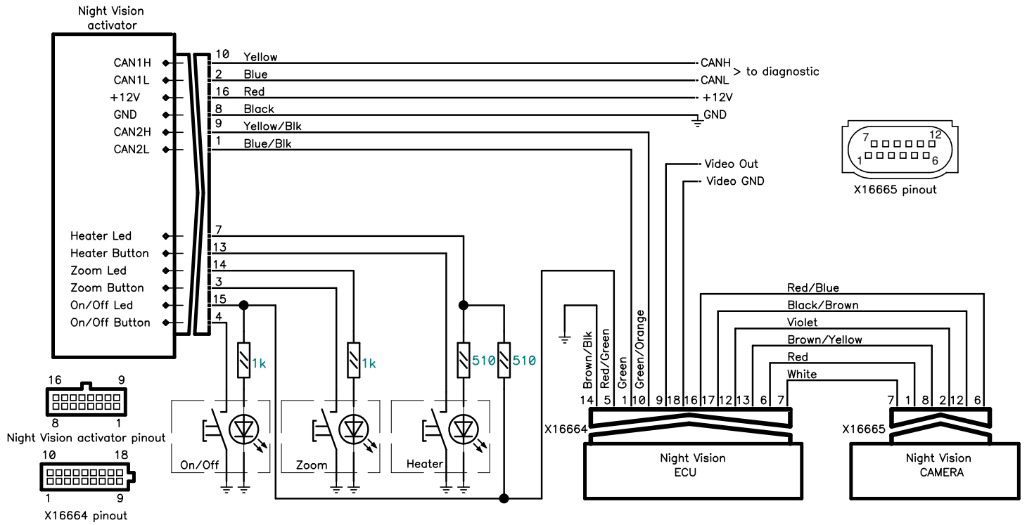
Pict 1. BMW E6X NiVi System Connection Diagram
